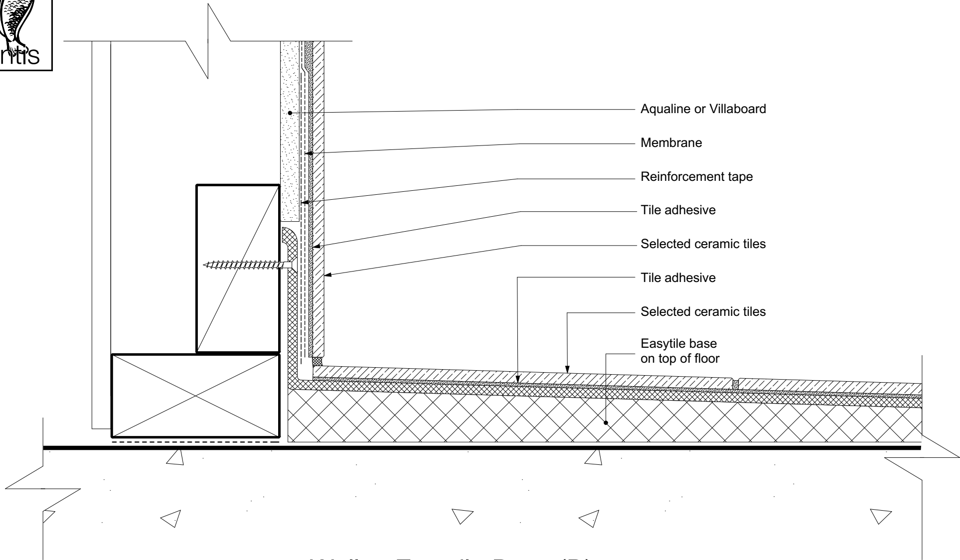
Wall to Easytile Base (B)
