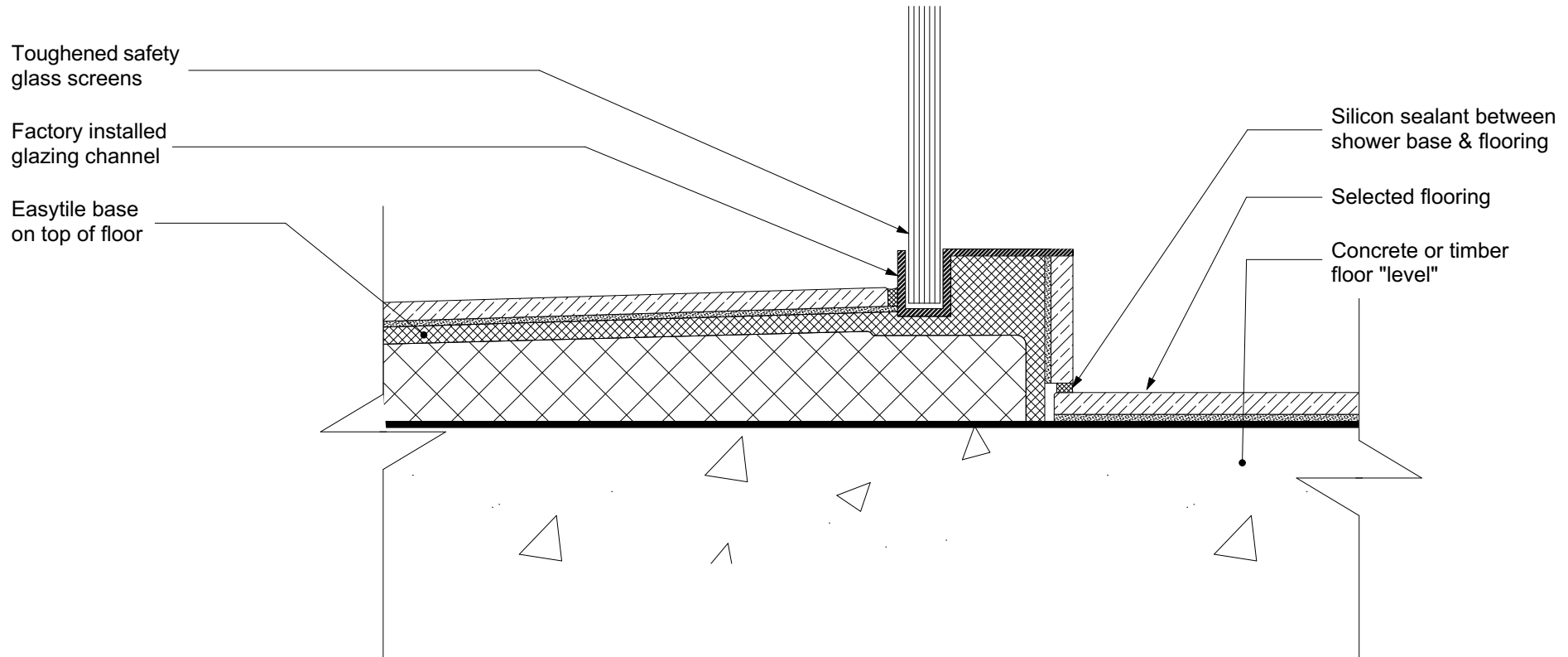
Floor to Easytile Base (C)
